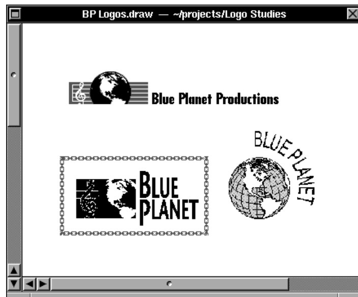
Figure 6-15 Linked Information
