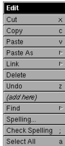
Figure 6-12 Edit Menu
