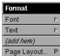
Figure 6-17 Format Menu
