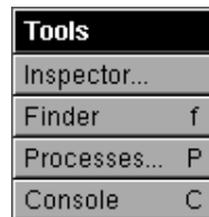
Figure 6-24 Tools Menu
